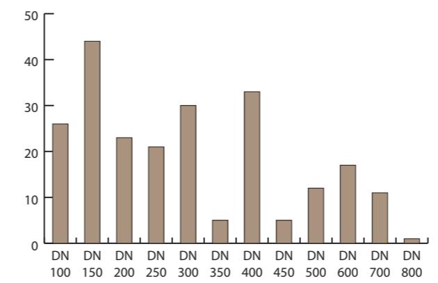
Number of HDD operations by DN
