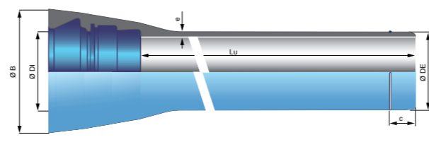
TT ZMU – DN 100 to DN 700
